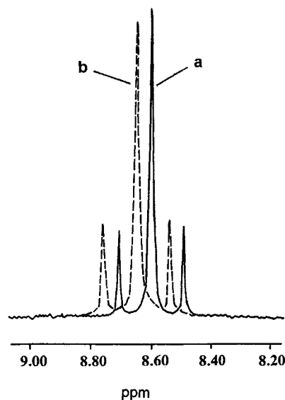
Figure 3. Representative ^1\text{H} NMR spectra of the N-protons of PT and [ ^{15}\text{N} ]PT recorded in acetone- d_6 . The samples were obtained by partial oxidation of a mixture of 35 mg of PT and 15 mg of [ ^{15}\text{N} ]PT and then separation of the neutral molecules (phase 1) and radical cations (phase 2). The latter was reduced to neutral molecules for NMR determination (see Experimental section for details). (a) Spectrum of phase 1 which shows a molar ratio of PT to [ ^{15}\text{N} ]PT of 1:2.54; (b) spectrum of phase 2 which shows a molar ratio of PT to [ ^{15}\text{N} ]PT of 1:2.16. Spectrum (b) is shifted downfield for clarity. K=0.85 for reaction (4) is obtained from this particular experiment
